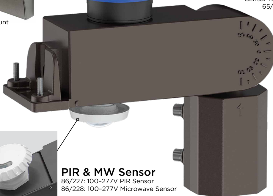
Extended Slip-Fitter with Sensor Knockouts 65/875
