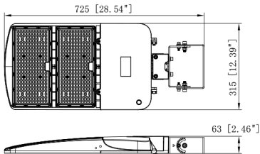
65/872 Trunnion Mount
