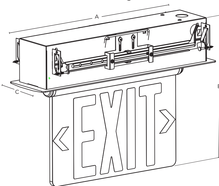
Recessed Ceiling Mount
